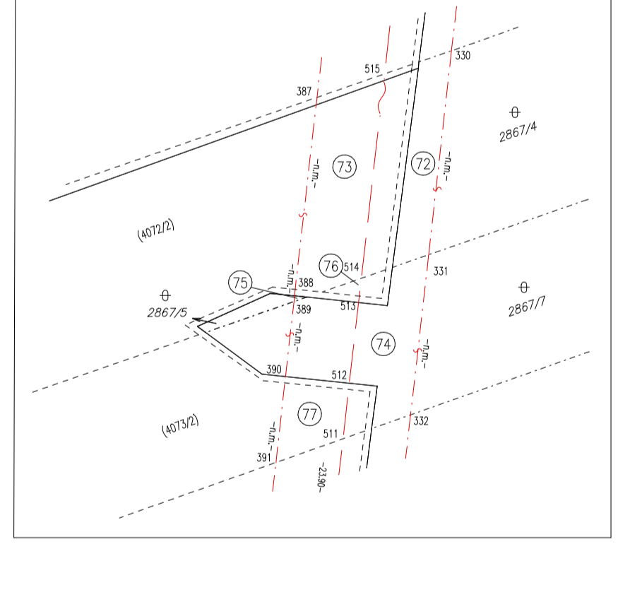
DETAIL "A"
