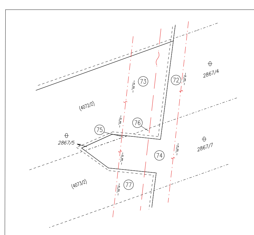
DETAIL "A"
